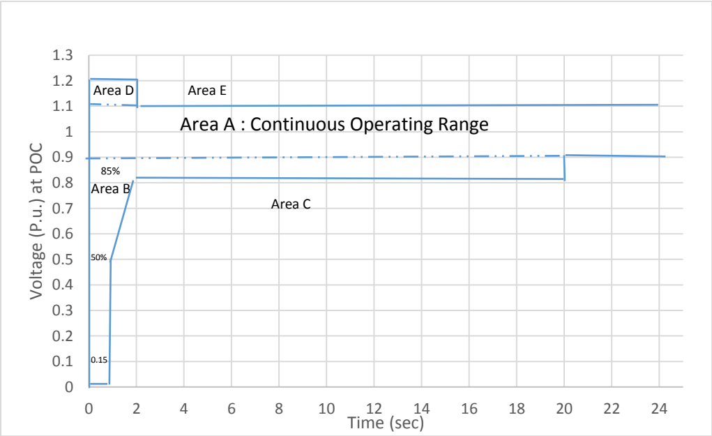
Figure 7-5: Voltage Ride through Capability for the RPPs utilising synchronous machines
