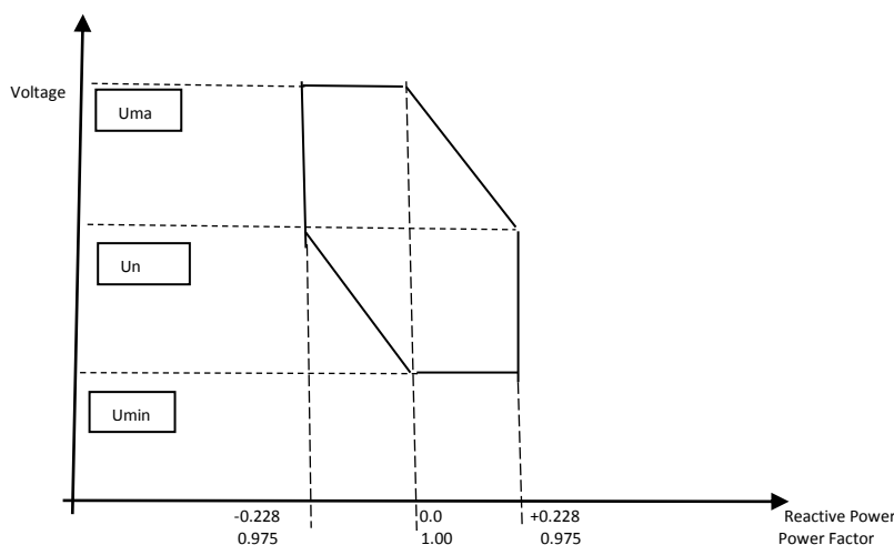
Figure 7-12: Requirements for reactive power and voltage control range for RPPs up to 20 MVA
