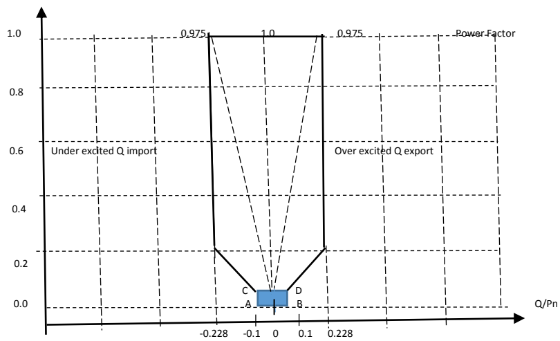
Figure 7-11: Reactive power requirements for RPPs (up to 20 MVA) at Nominal Voltage at POC
