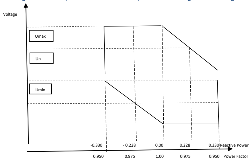
Figure 7-15: Requirements for reactive power and voltage control range for RPPs above 20 MVA
