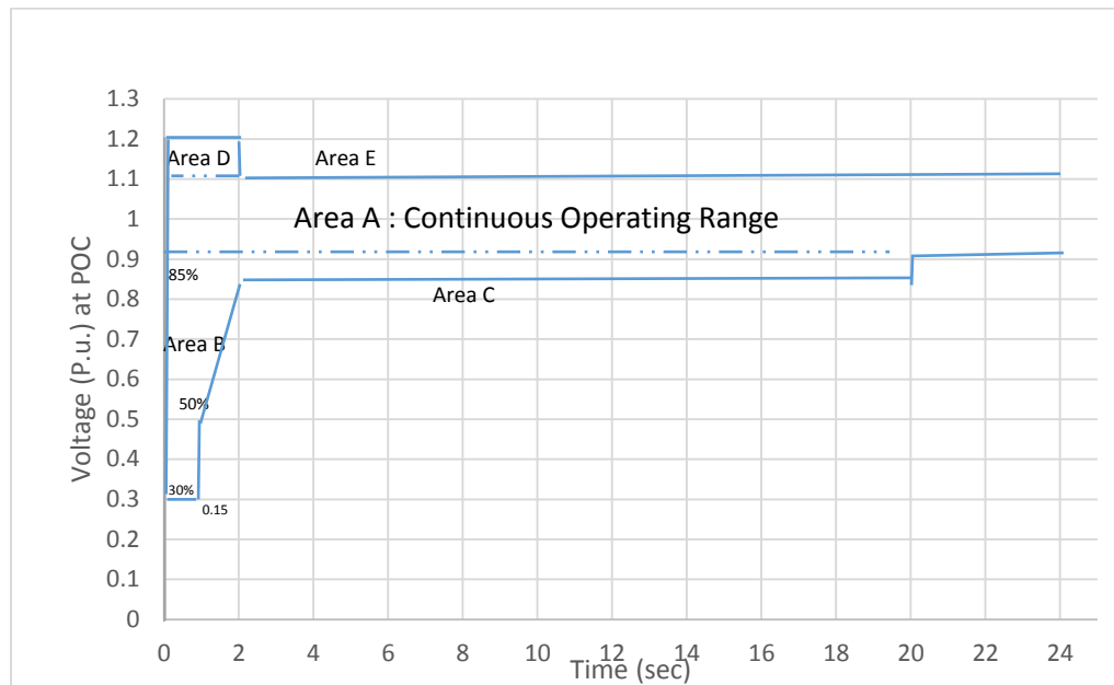
Figure 7-6: Voltage Ride through Capability for the RPPs (up to 20 MVA) utilizing synchronous machines (three phase faults only)
