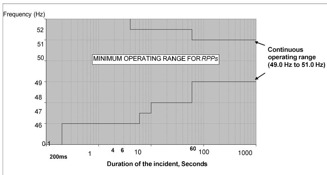
Figure 7-3: Minimum frequency operating range of RPP (during a system frequency disturbance)
