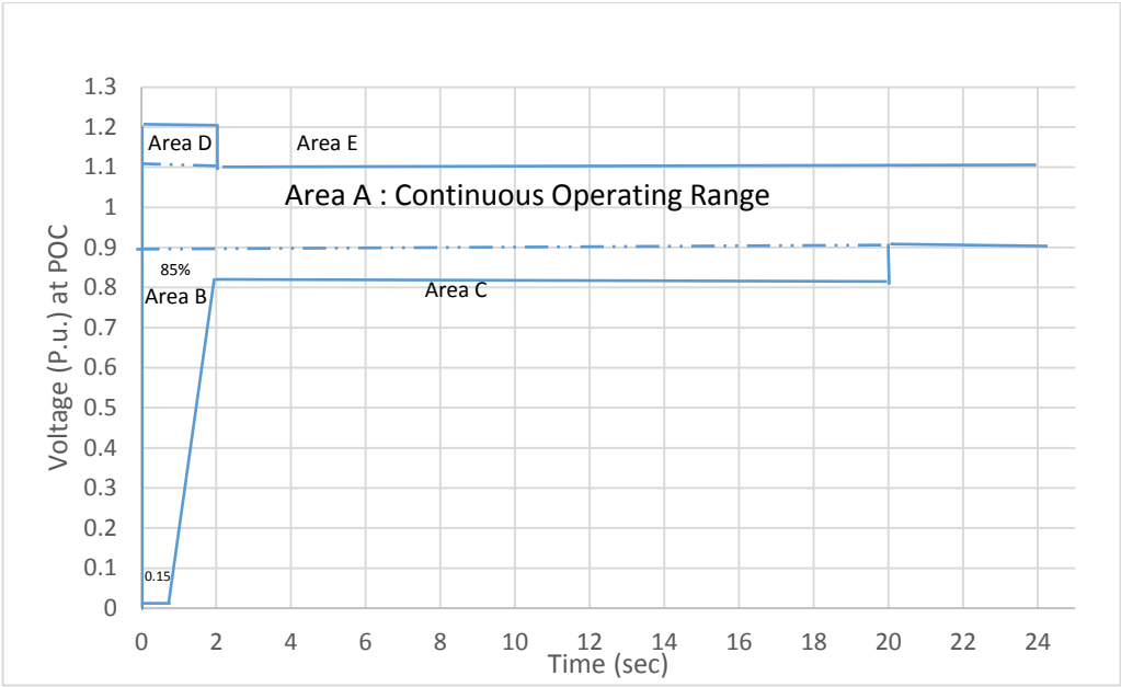
Figure 7-4: Voltage Ride through Capability for the RPPs utilising non-synchronous machines
