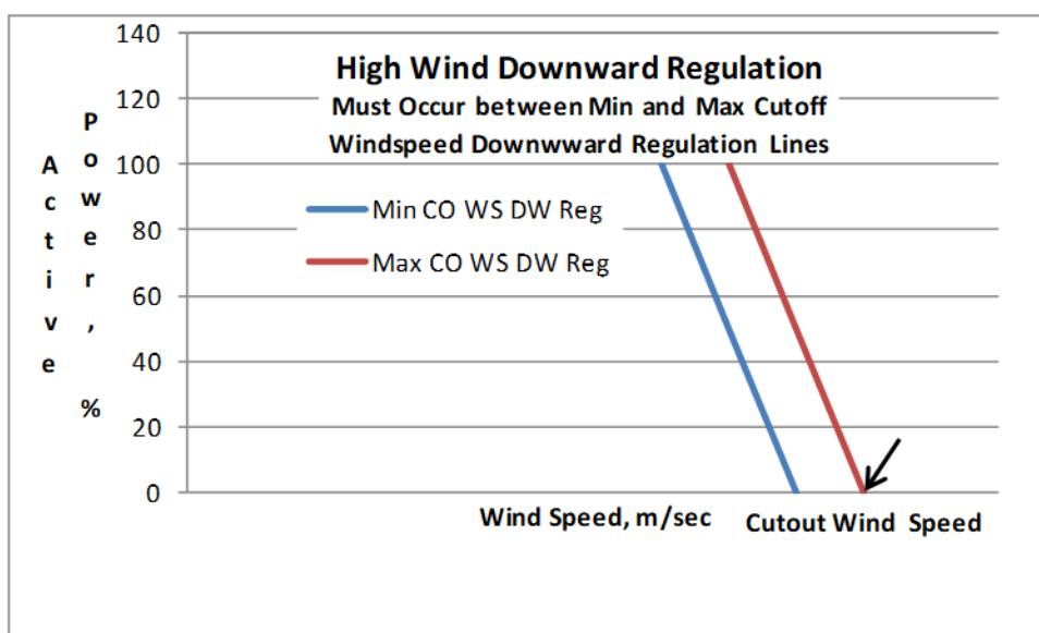
Figure 7-19: Illustrative High Wind Downward Regulation Chart
