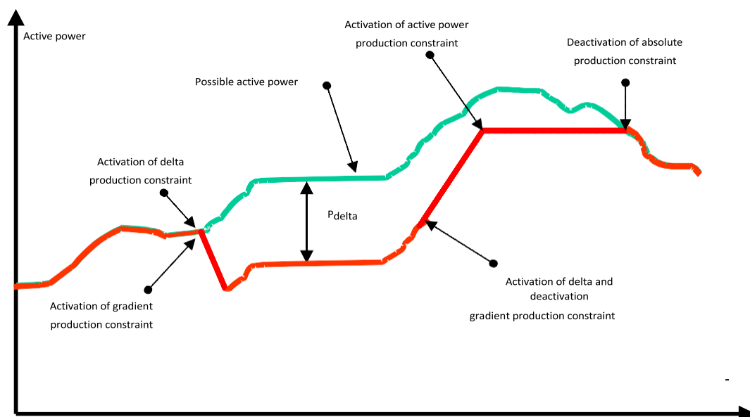
Figure 7-18: Active power control functions for a Renewable Power Plant
