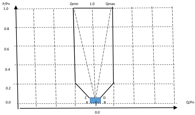
Figure 7-10: Reactive power requirements for RPPs (size up to 20 MVA) at POC
