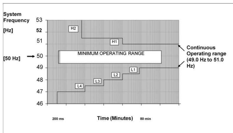
Figure 7-2: Minimum frequency operating range for RPP
