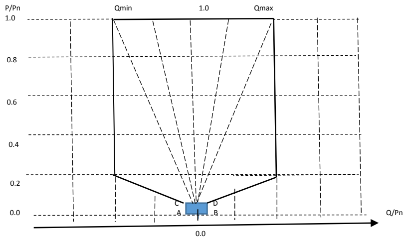
Figure 7-14: Requirements for reactive power and voltage control range for RPPs above 20 MVA (at nominal voltage at POC)
