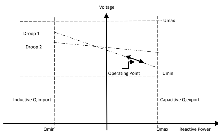
Figure 7-17: Voltage Control for RPP
