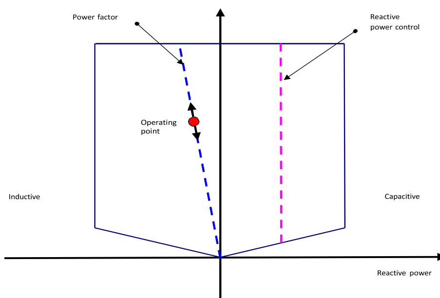
Figure 7-16: Reactive Power Control for RPP
