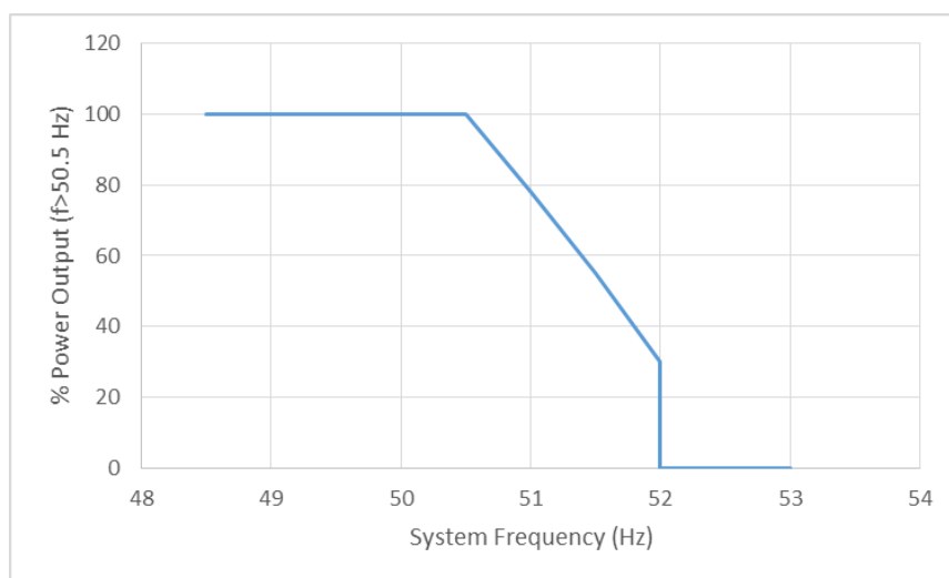
Figure 7-8: Power curtailment during over-frequency for RPPs
