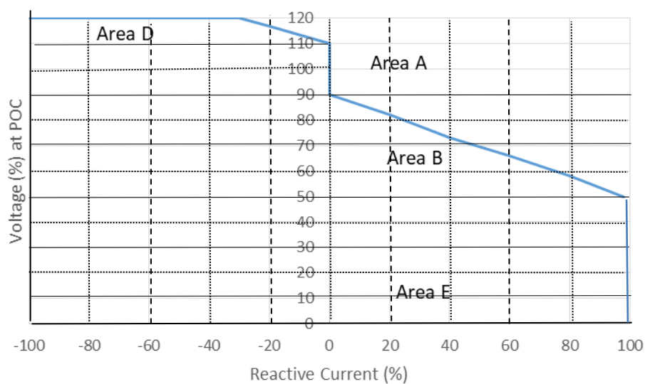
Figure 7-7: Requirements for Reactive Power Support, I_Q , during voltage drops or peaks at the POC
