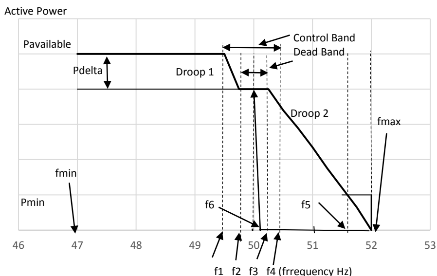
Figure 7-9: Frequency response requirement for RPPs of size above 20 MVA
