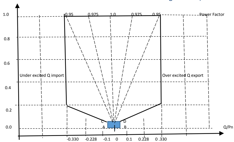
Figure 7-14: Requirements for reactive power and voltage control range for RPPs above 20 MVA (at nominal voltage at POC)
